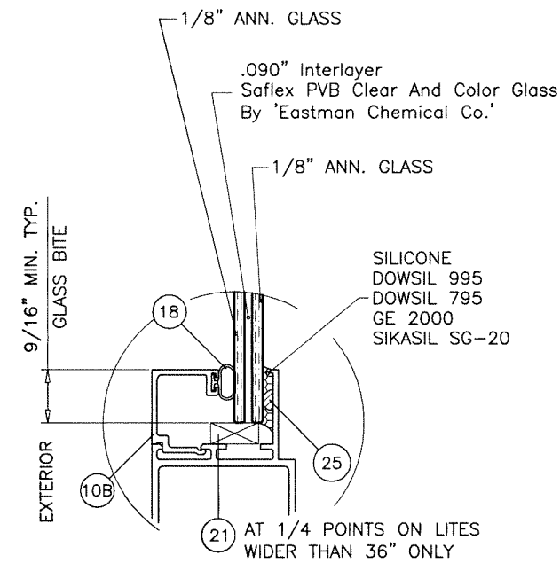
GLASS TYPE 'C' 5/16" OVERALL LAM. GLASS
